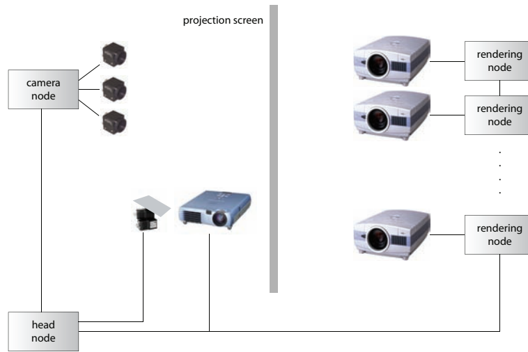
Figure 3: System configuration.
